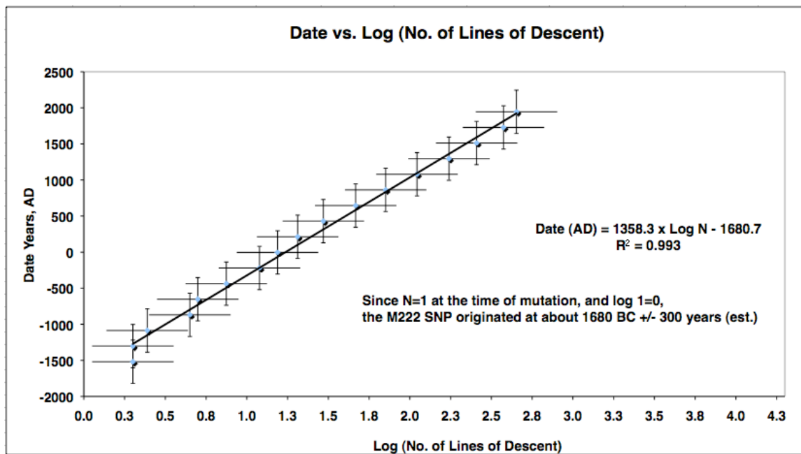
Figure 3: Date vs. Log of the Number of Lines of Descent in Two Well-Populated Phylogenetic Trees (The error bars (SD) on each point are the log (square root of the counted number of lines) and 300 years)
