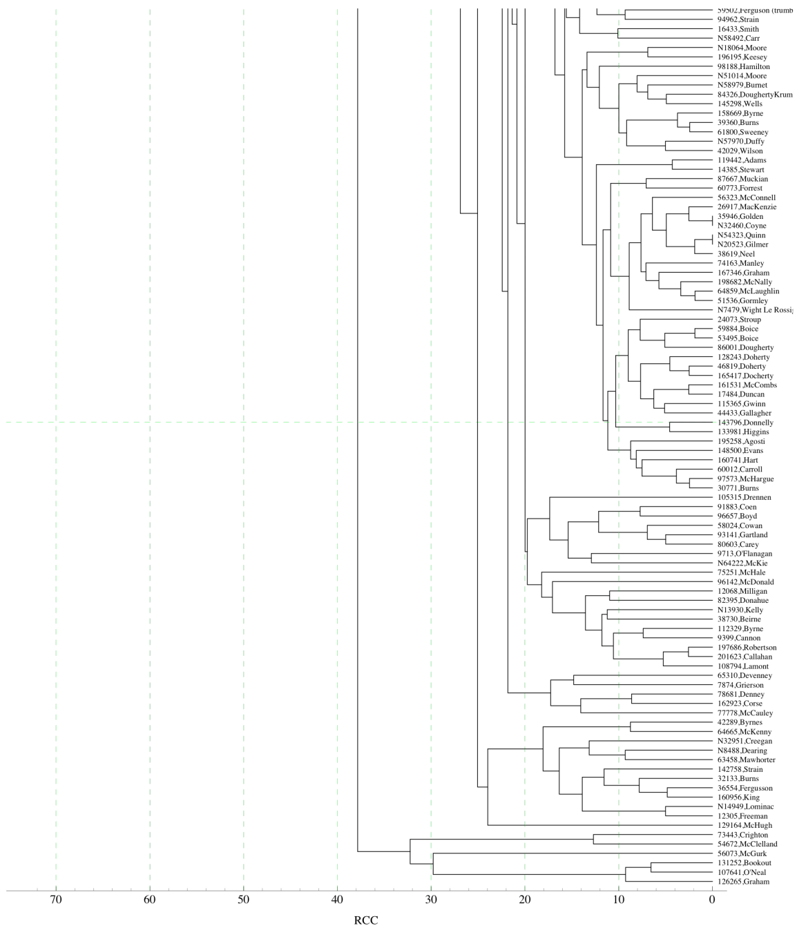
Figure 2: The Phylogenetic Tree Generated from 184 37 Marker Haplotypes of Sixteen Similarly-Spelled or -Prefixed Surnames That Are Tightly Clustered.
